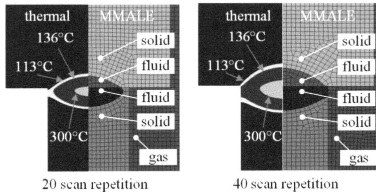
Fig. 2 Precomputed temperature field using ANSYS and the MMALE-Model with fluid and solid parts at two different scan repetitions (left and right).
