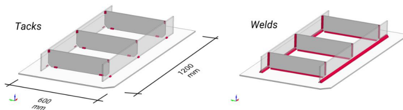
Fig. 2 Dimension, tack welds and welds of test specimen
