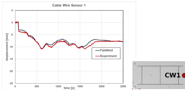
Fig. 8 Result cable wire sensor 1
