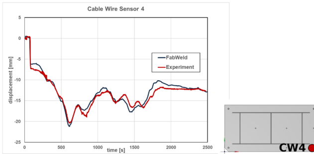
Fig. 11 Result cable wire sensor 4
