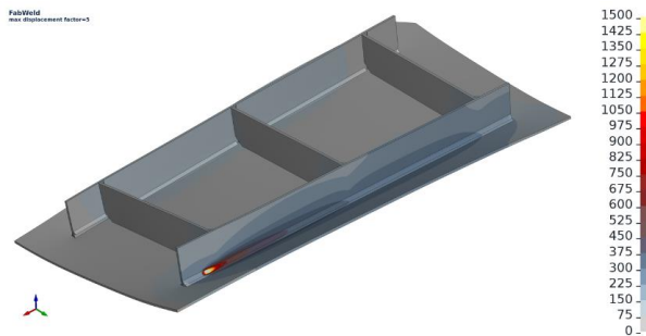
Fig. 7 Temperature displayed on 5-times magnified deformed structure
