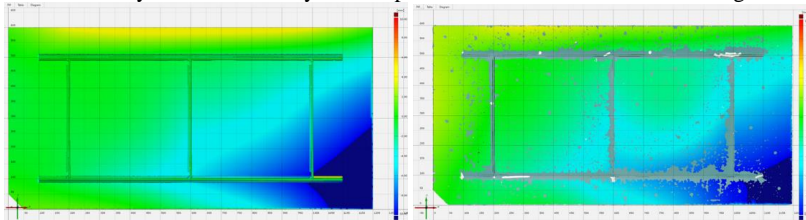
Fig. 14 Surface deviation. Left simulation, right experiment
