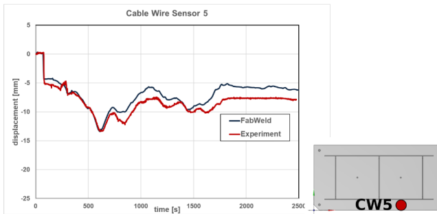
Fig. 12 Result cable wire sensor 5
