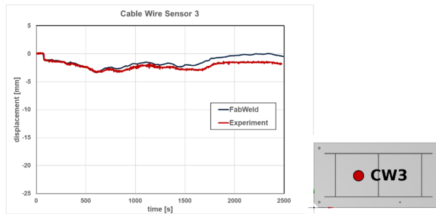
Fig. 10 Result cable wire sensor 3
