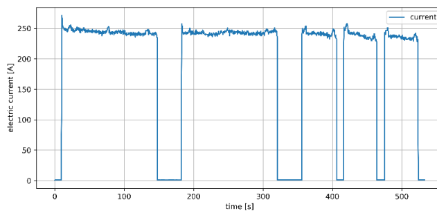
Fig. 5 Electrical current during welding
